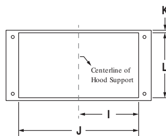
CUTOUT VIEW
