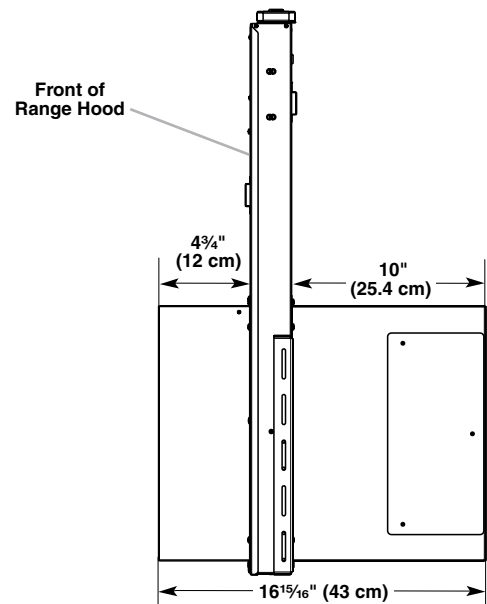
Reversed Blower
