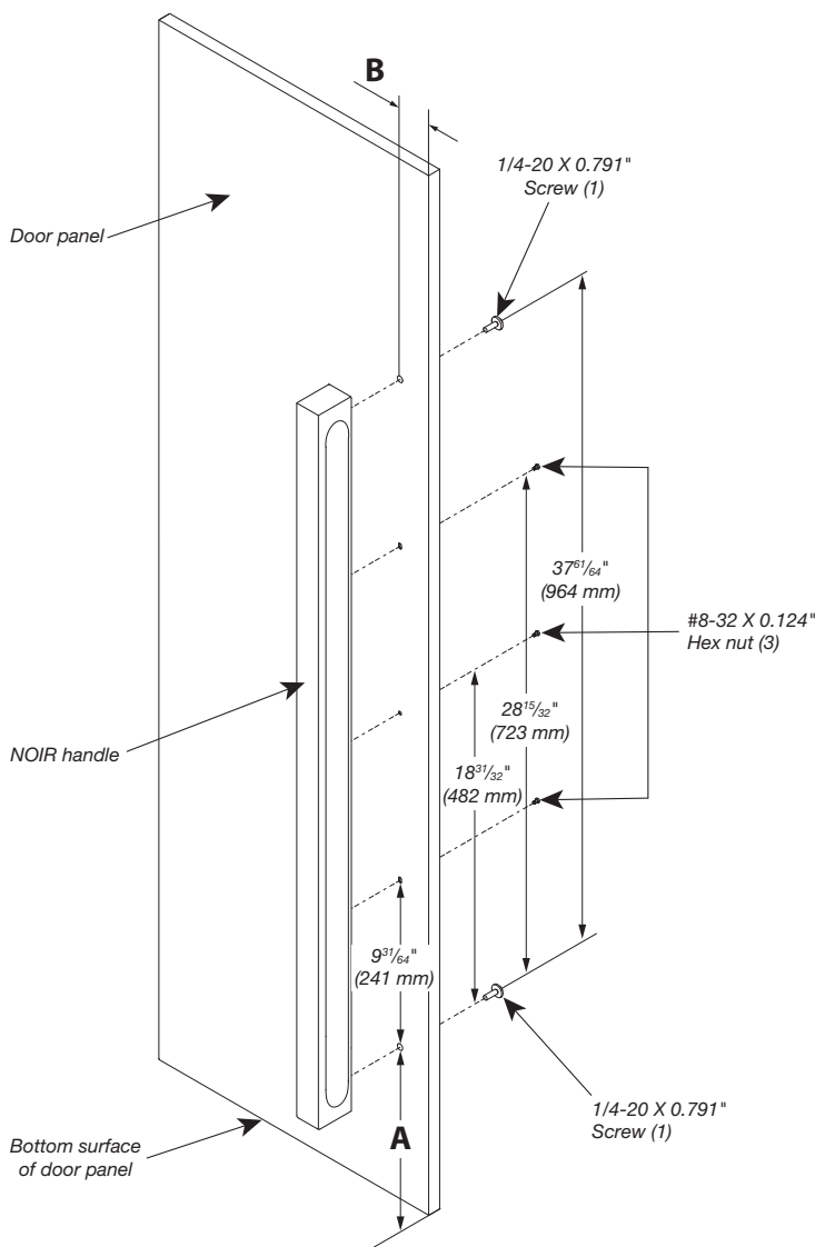
Figure 1 - Refrigerator/freezer door
