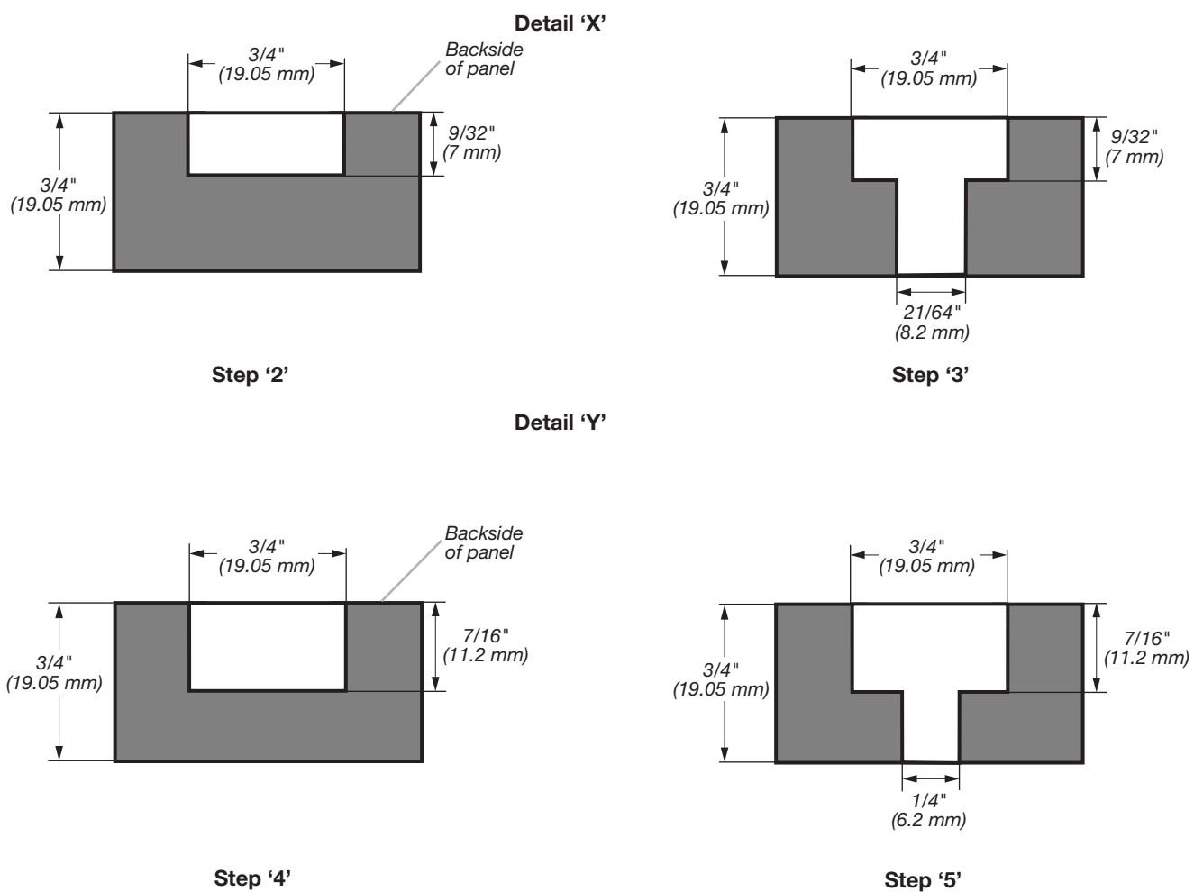
Figure 5 - Cross sectional view
