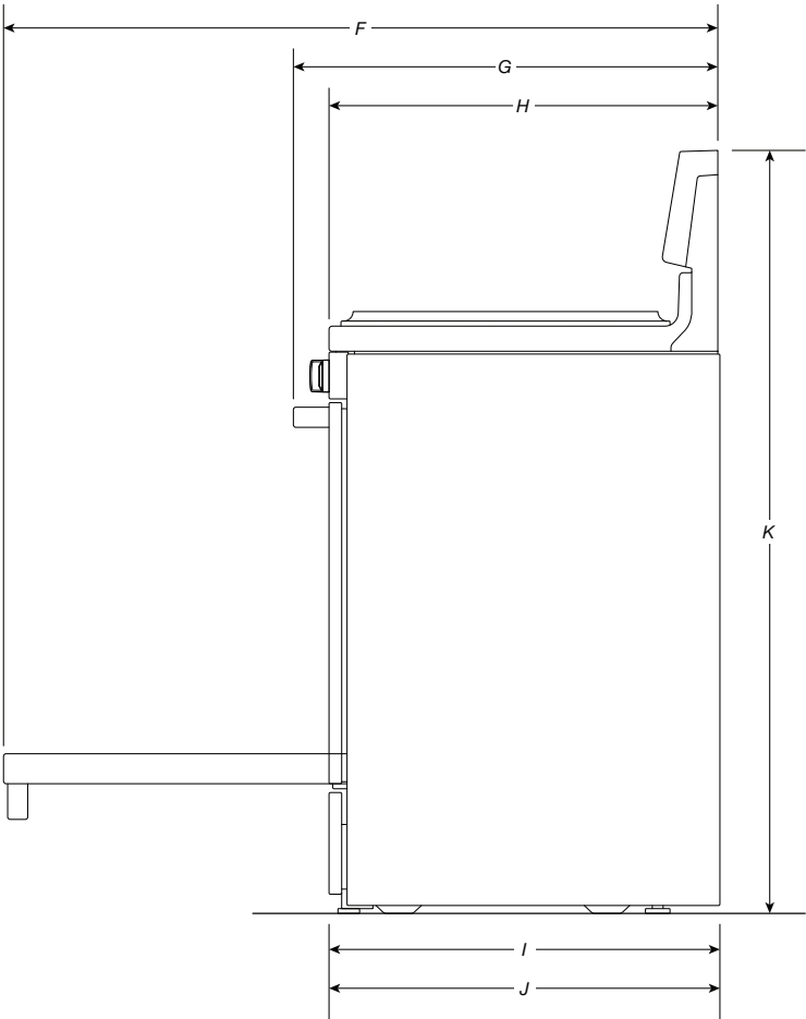
SIDE VIEW
