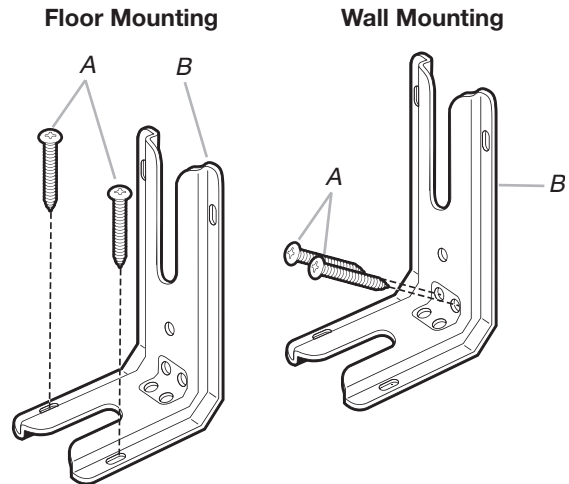
A. #12 x 1\frac{5}{8} " screws B. Anti-tip bracket
